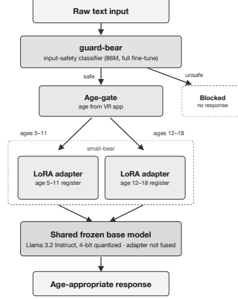
Fig. 1 System architecture diagram. The guard-bear safety layer (86M parameters) screens incoming text before routing safe queries to age-stratified LoRA adapters deployed on a frozen 4-bit Llama 3.2 base model.
