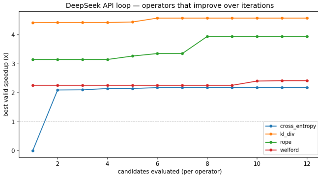
Fig. 4. Per-iteration optimization progress (DeepSeek API loop): best-so-far speedup vs. candidates evaluated, for the focus operators whose search visibly improves over iterations (flat-from-first-success operators omitted). cross_entropy is repaired at candidate 2; rope climbs via a structural improvement around candidate 8.
