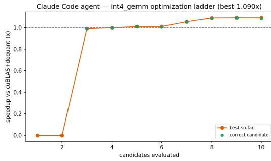
Fig. 4. Claude Code agent on int4_gemm : best-so-far speedup over a cuBLAS+dequantize baseline. Two failed attempts, then a correct kernel and a tuning ladder to 1.09 \times .
