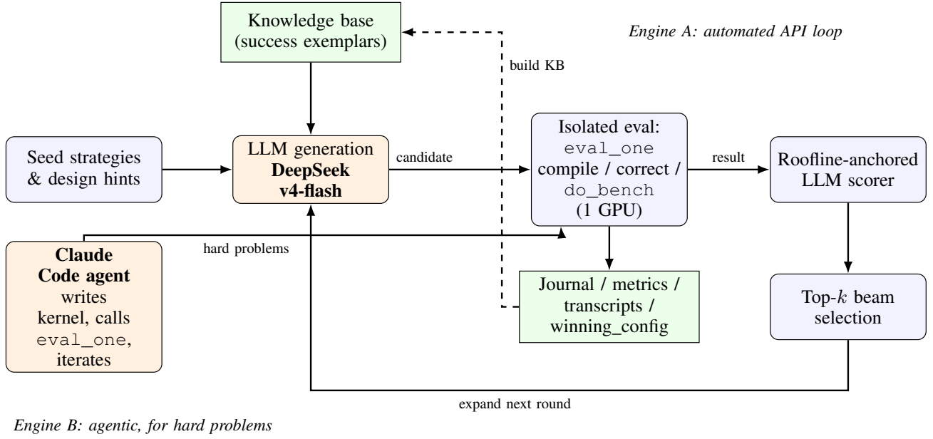
Fig. 1. The closed-loop harness. Engine A (DeepSeek API loop) and Engine B (Claude Code agent) are two entry points into one shared evaluator; all persisted artifacts (logs, transcripts, winning configurations) are produced by the evaluator, not the generator.
