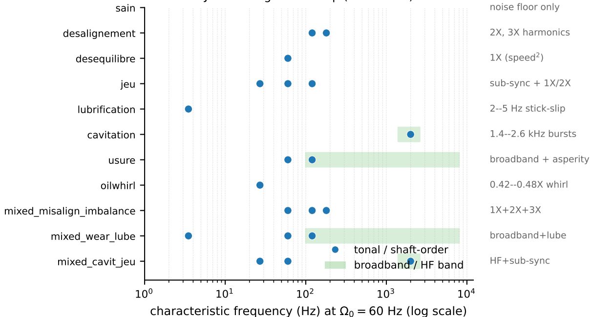
JBFD-11 signature map (11 classes)
