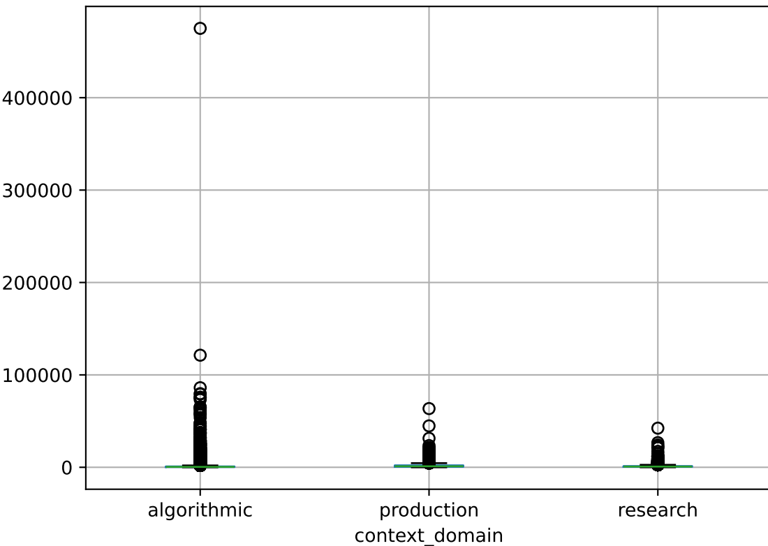
Code Length by Domain
