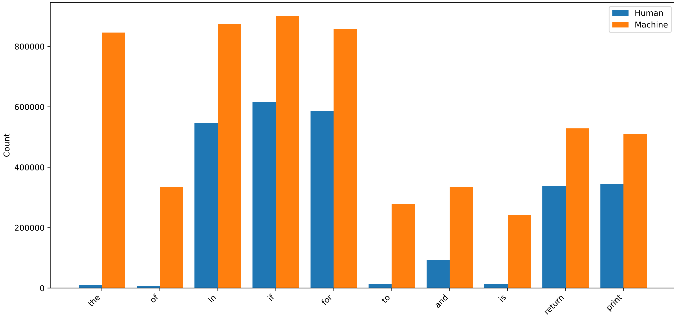
Top 10 n-grams More Frequent in Machine-Generated Code
