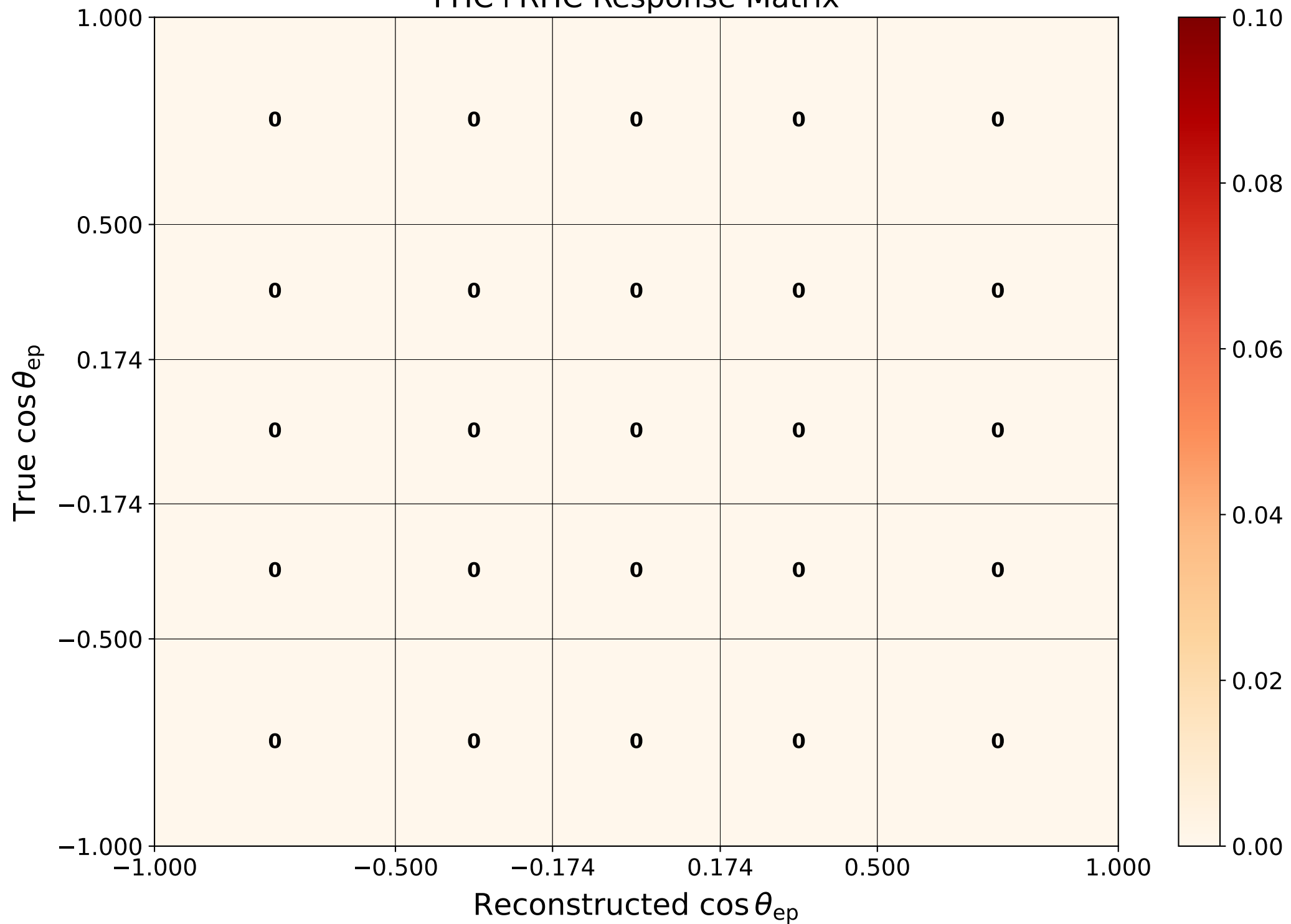
FHC+RHC Response Matrix
