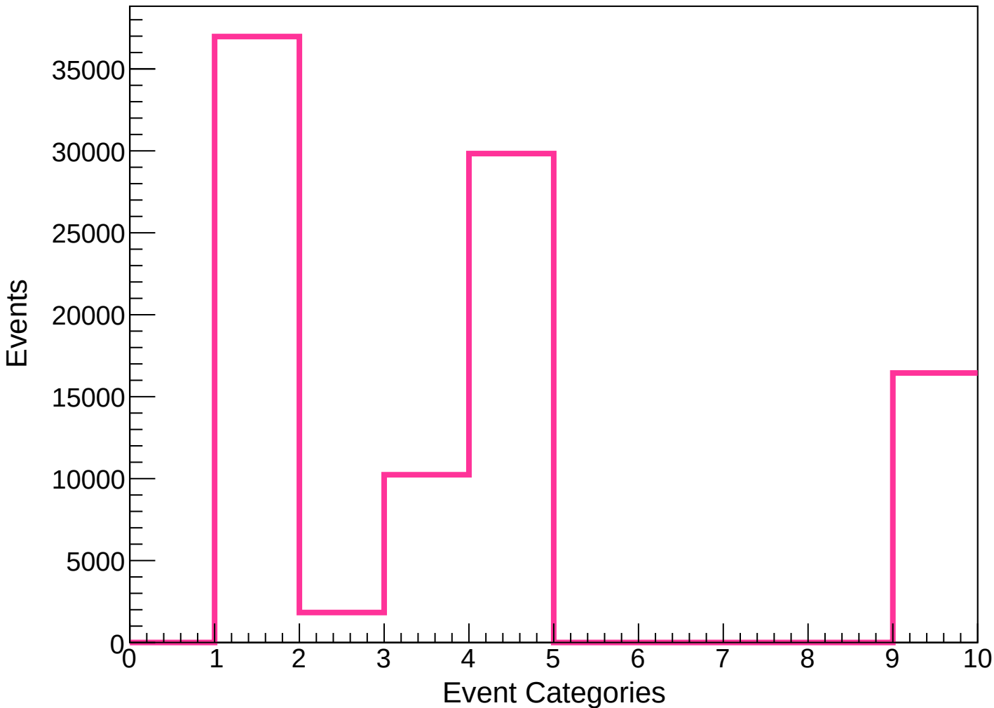
NuMI Run 1 FHC Event Categories (Intrinsic Nue)
