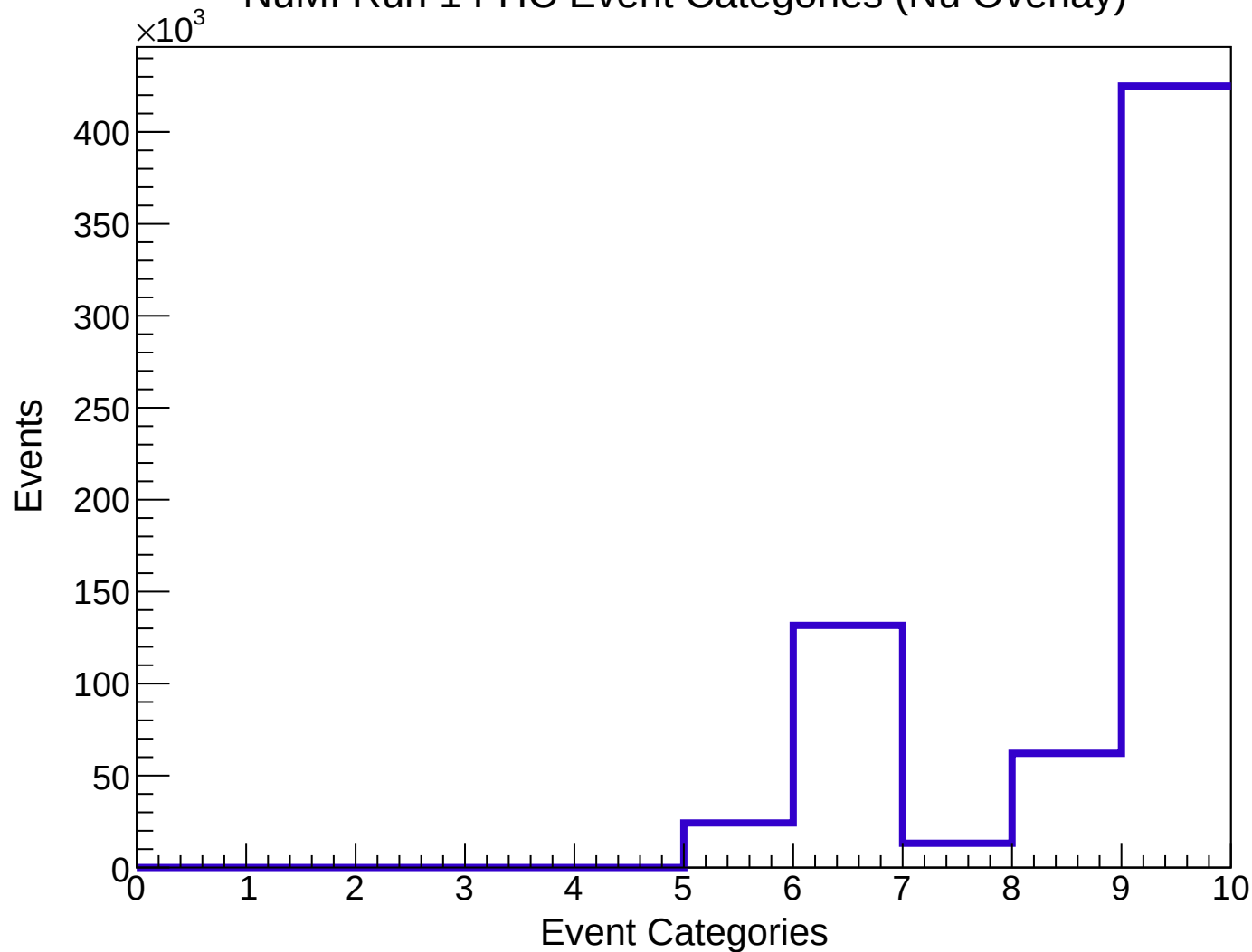
NuMI Run 1 FHC Event Categories (Nu Overlay)
