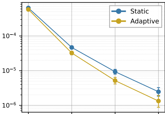
(a) Logical error rate
