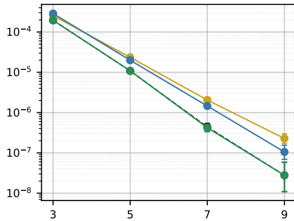
(b) Logical error rate
