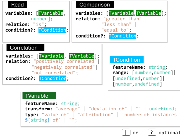
Figure 2: Schema of the Structured Insight Format. The three insight types, i.e. , Read, Comparison, and Correlation, are specified by variables, relations, and optional conditions. Each variable (TVariable) and condition (TCondition) follows a consistent format to support structured parsing. The schema follows the type definition syntax in TypeScript.
