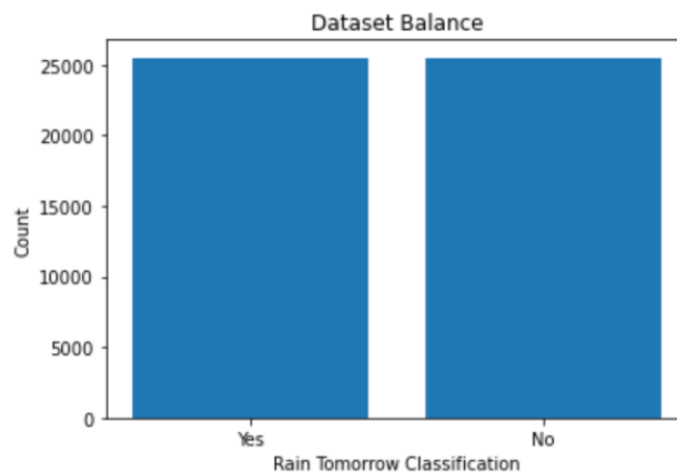
After Undersampling:
