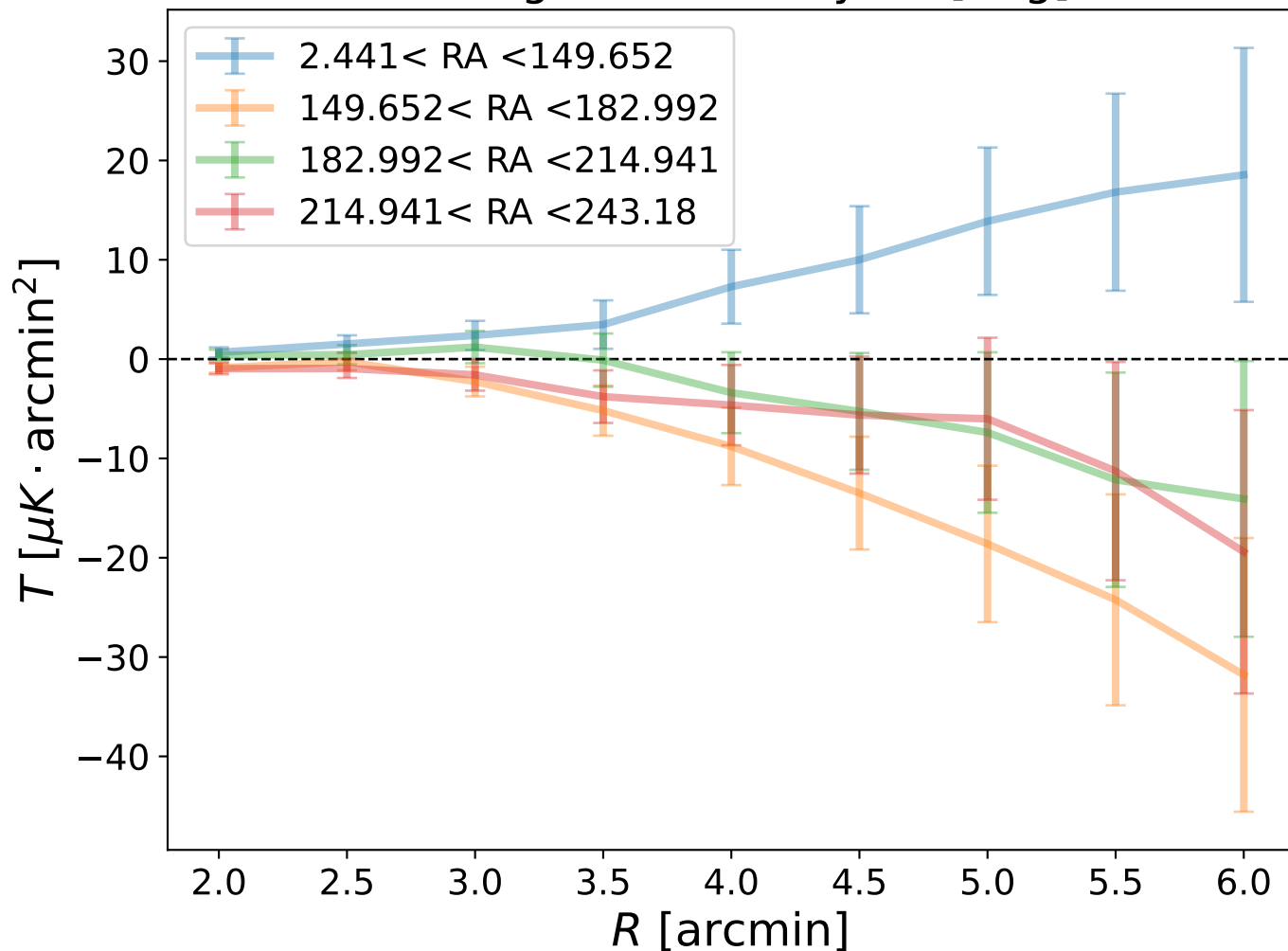
tSZ signal binned by RA [deg]
