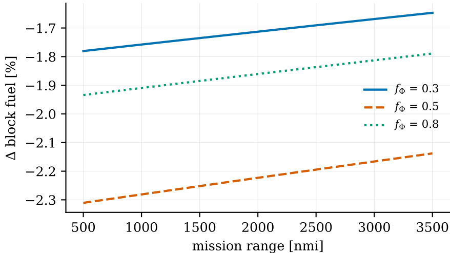
turboelectric chain, FPR 1.25, snowball 1.35
