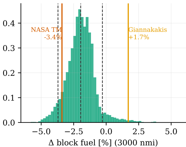
(b) block-fuel delta with literature estimates
