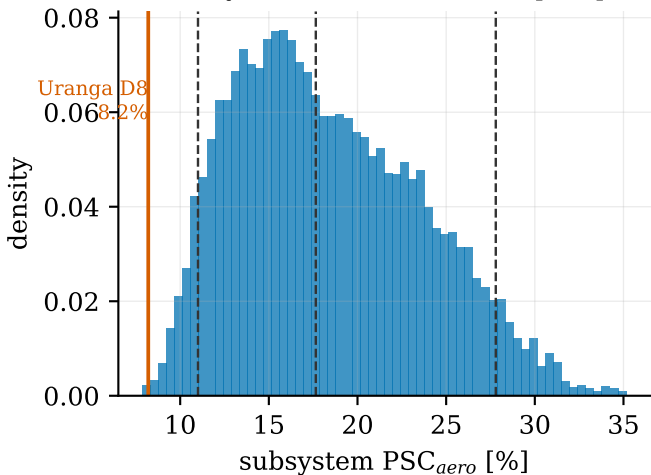
(a) aerodynamic PSC across the input space
