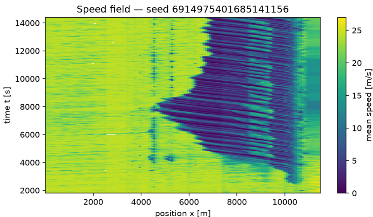
Space-time mean-speed contour, seed 6914975401685141156
