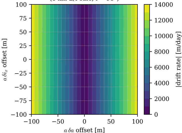
Drift rate vs element offsets (1 km E/I-safe, i = 98^\circ )
