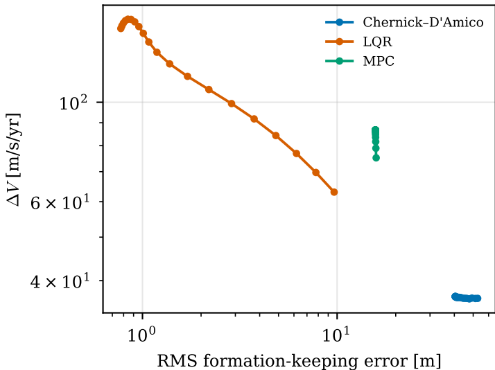
Perfect-navigation Pareto (1 km E/I-safe, i = 98^\circ )
