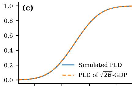
Under Q
