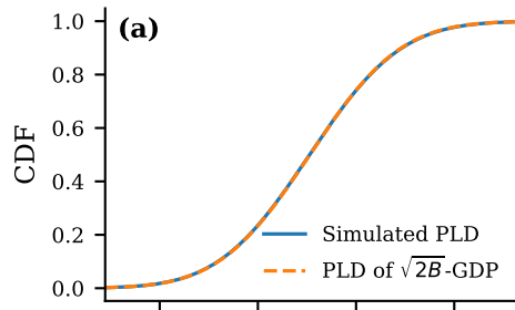
Under P
