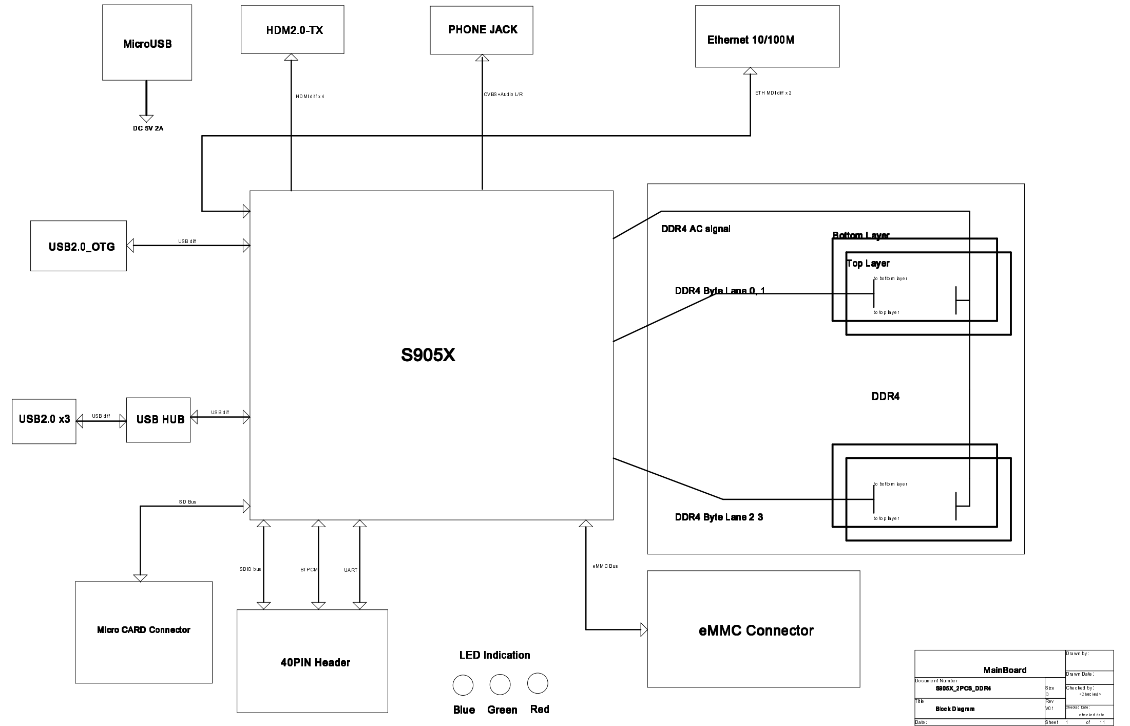
Block Diagram of S905X_2PCS_DDR4
