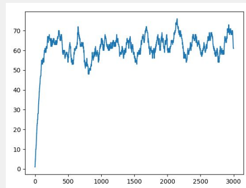
Training Score per episode (pt.2)
