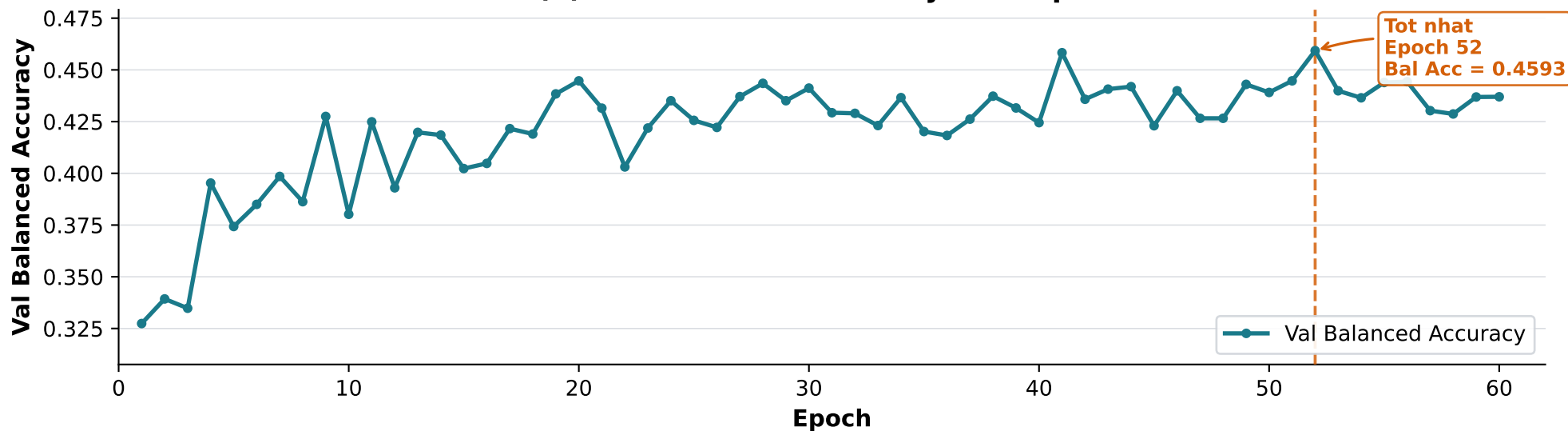
(b) Val Balanced Accuracy theo Epoch
