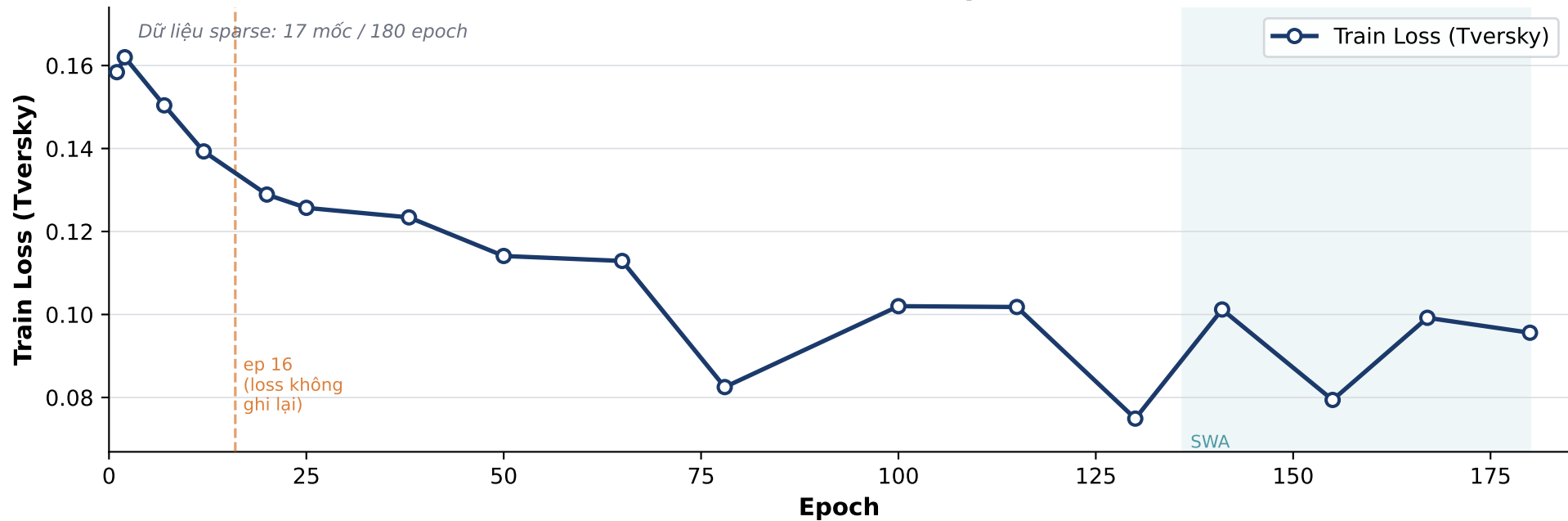
(a) Train Loss theo Epoch
