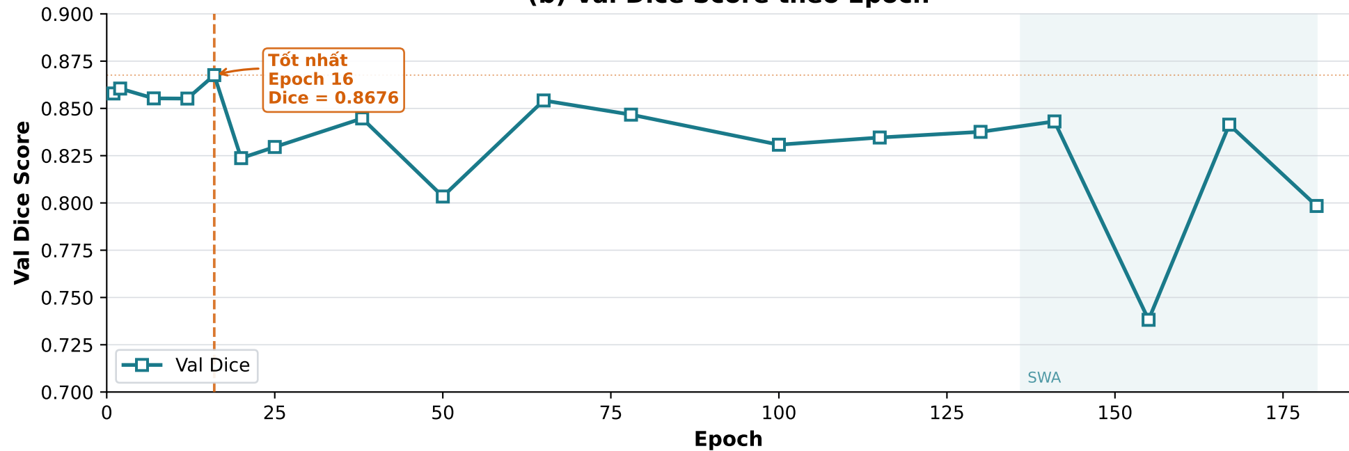
(b) Val Dice Score theo Epoch
