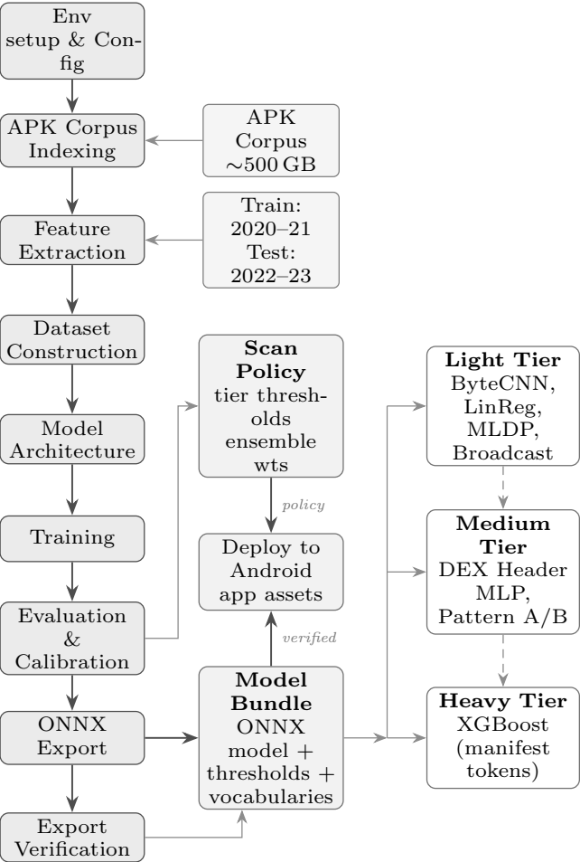
Fig. 1. Offline model-development pipeline.
