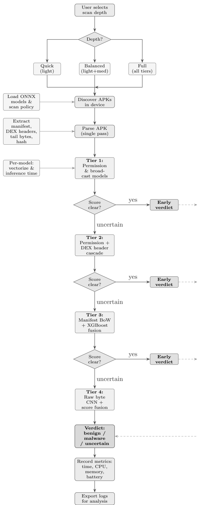
Fig. 2. VigiDroid on-device scanning flow. The app parses each APK once, then runs a tiered cascade of increasingly expensive models—exiting early when a confident score is reached—and logs per-stage resource metrics for thesis evaluation.
