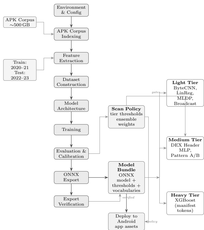
Fig. 1. Offline model-development pipeline. APKs are indexed, features extracted, models trained with temporal splits, and exported as verified ONNX bundles grouped into Light, Medium, and Heavy inference tiers.
