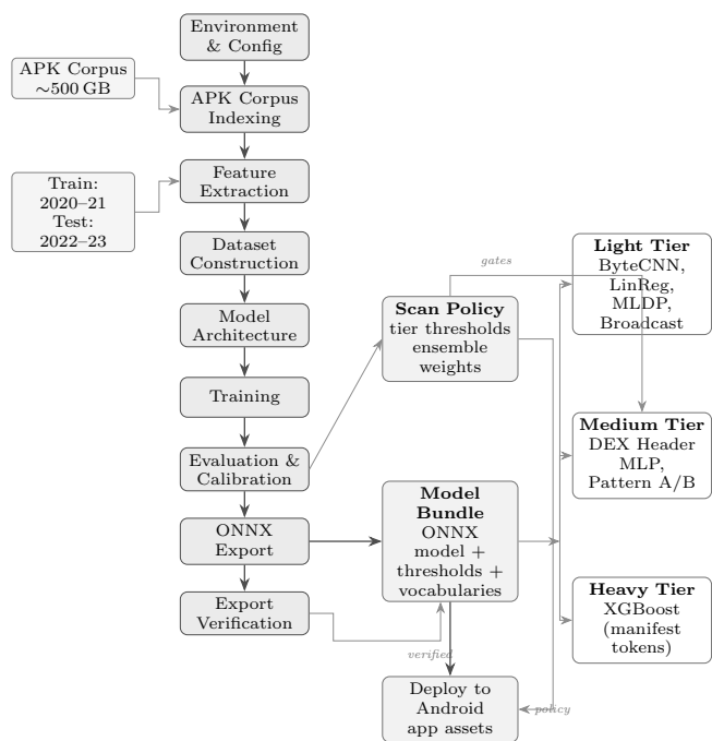
Fig. 1. Offline model-development pipeline. APKs are indexed, features extracted, models trained with temporal splits, and exported as verified ONNX bundles grouped into Light, Medium, and Heavy inference tiers.
