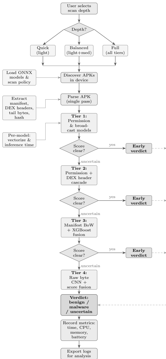
Fig. 2. VigiDroid on-device scanning flow. The app parses each APK once, then runs a tiered cascade of increasingly expensive models—exiting early when a confident score is reached—and logs per-stage resource metrics for thesis evaluation.
