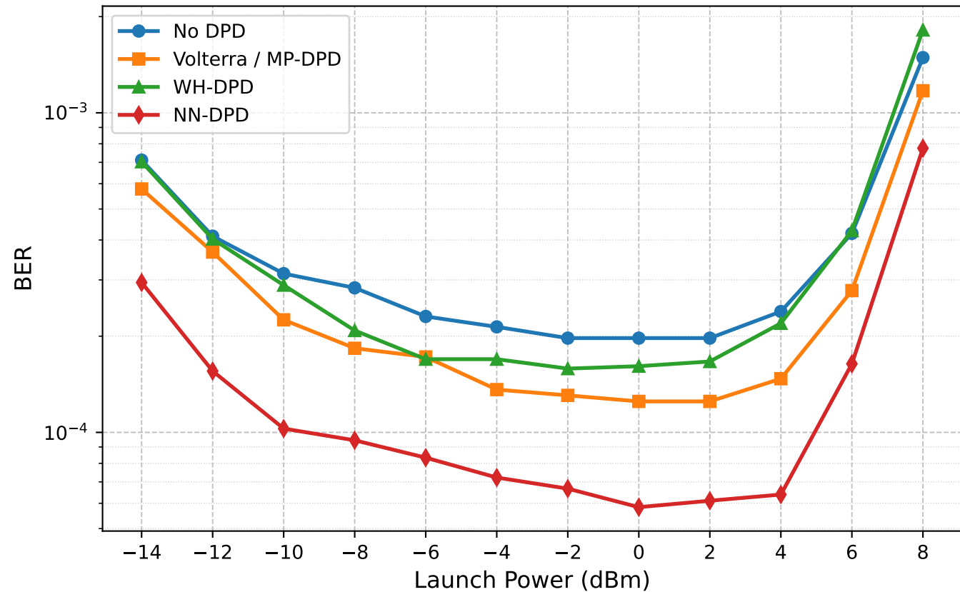
BER versus Launch Power for Different DPD Methods
