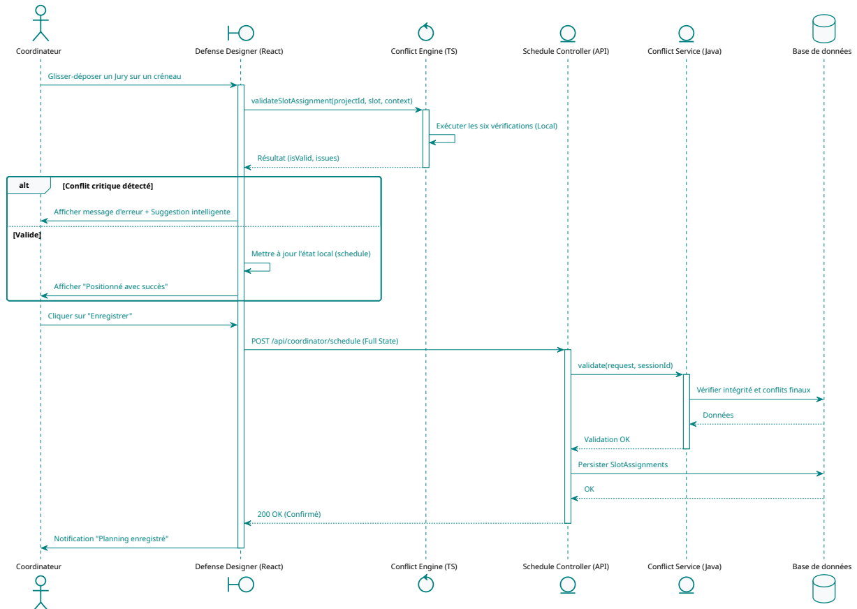
FIGURE 13 – Séquence de planification interactive via le Defense Designer
