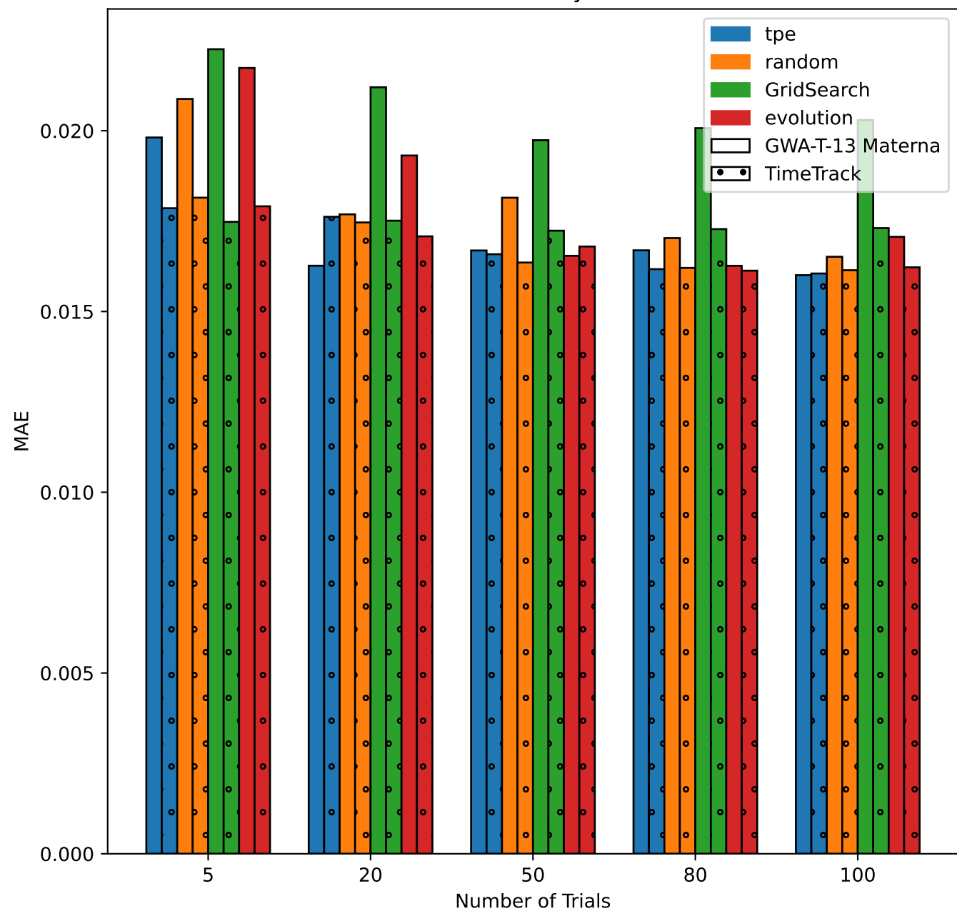
Minimum MAE vs. Number of Trials by Search Method and Dataset
