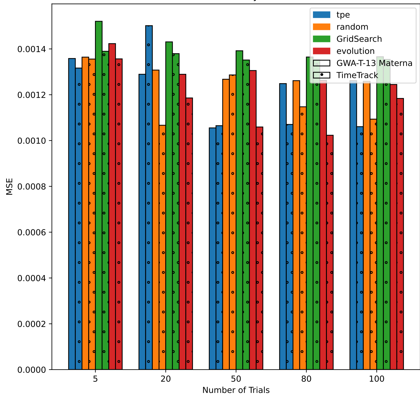
Minimum MSE vs. Number of Trials by Search Method and Dataset
