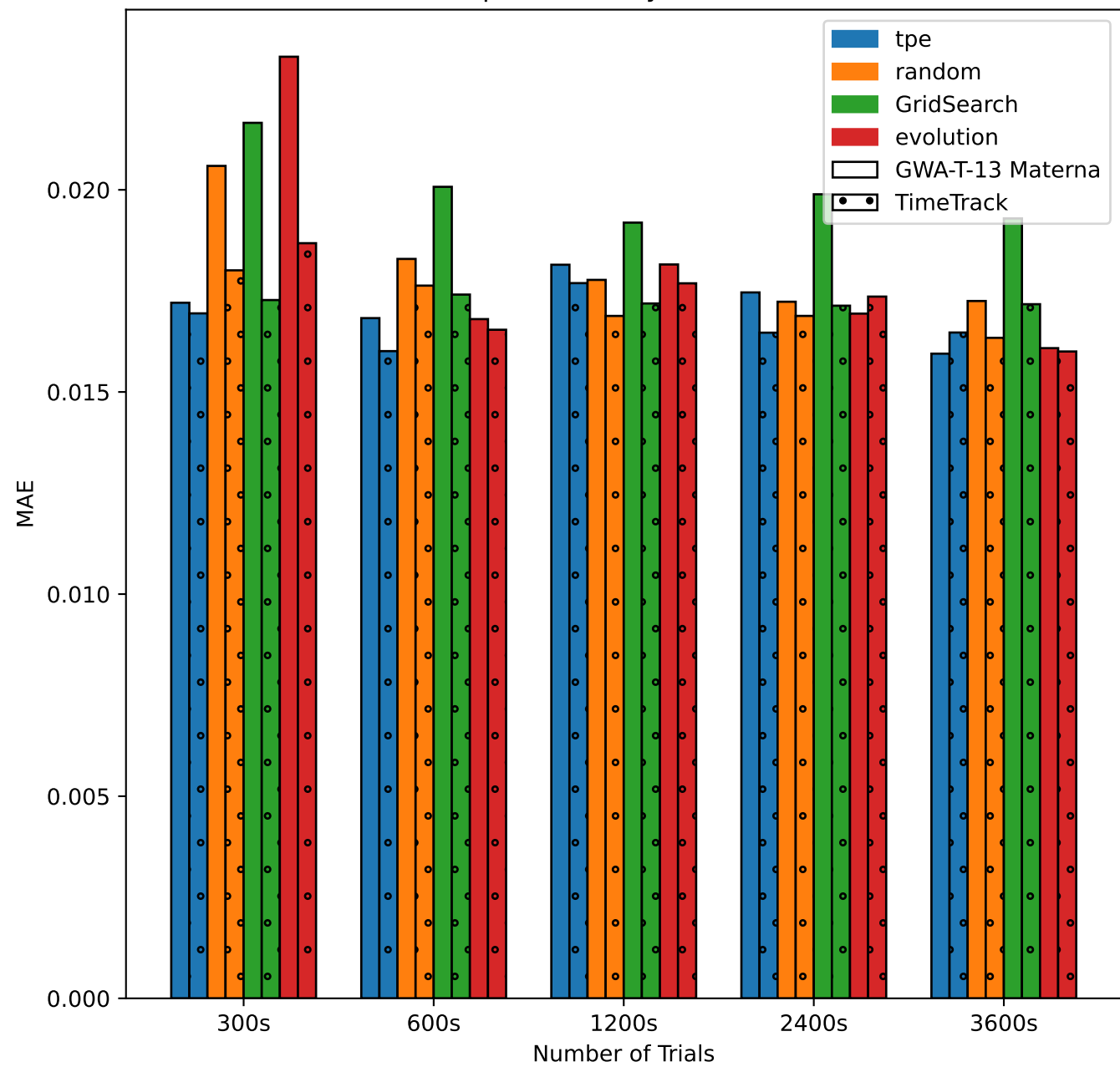
Minimum MAE vs. exp duration by Search Method and Dataset
