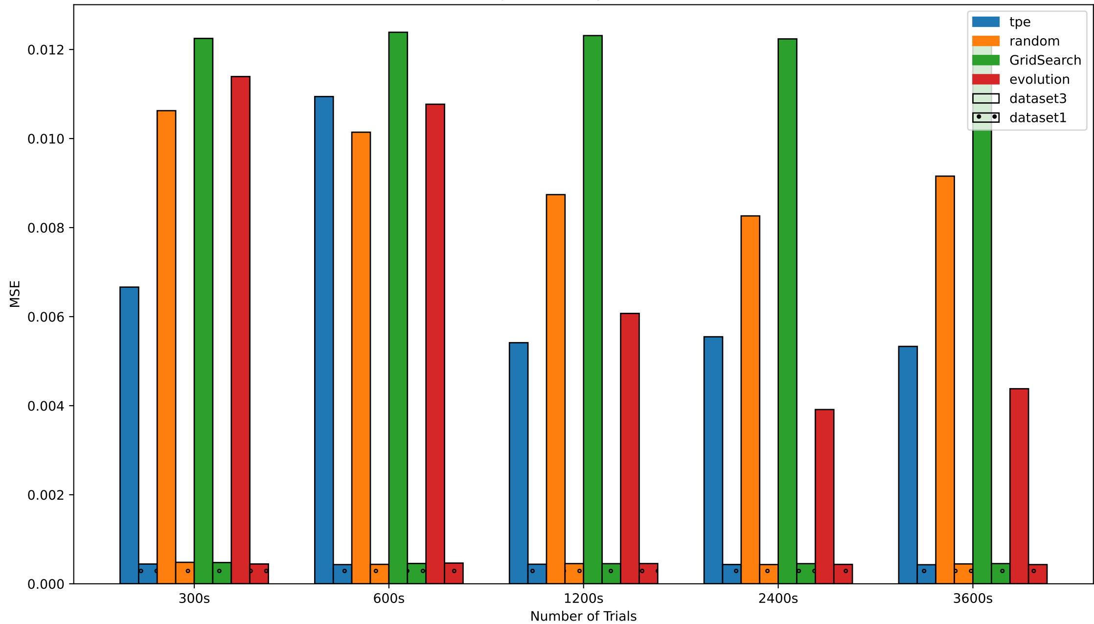
Minimum MSE vs. exp duration by Search Method and Dataset
