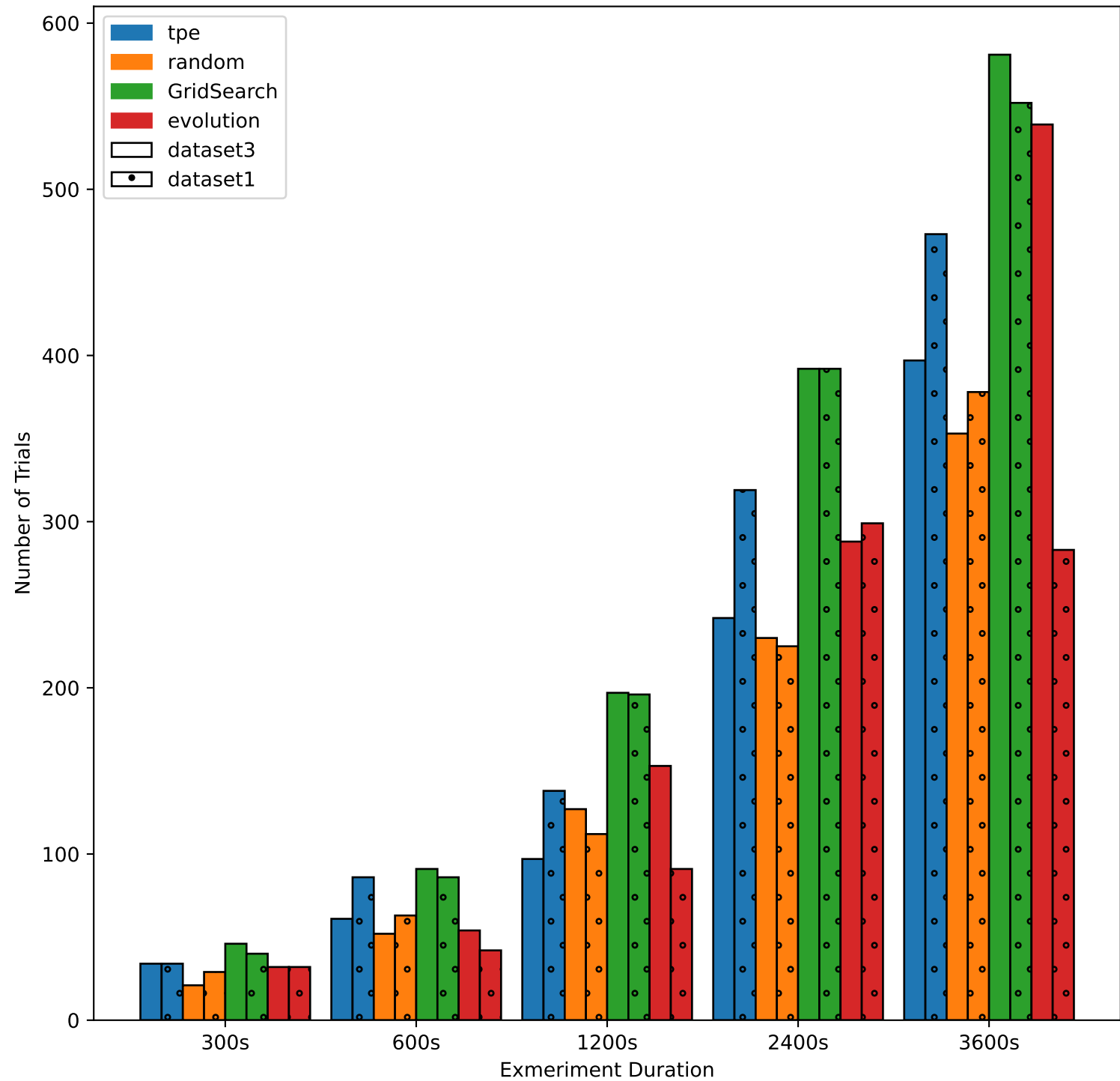
Number of trials vs. Expiriment duration by Search Method and Dataset
