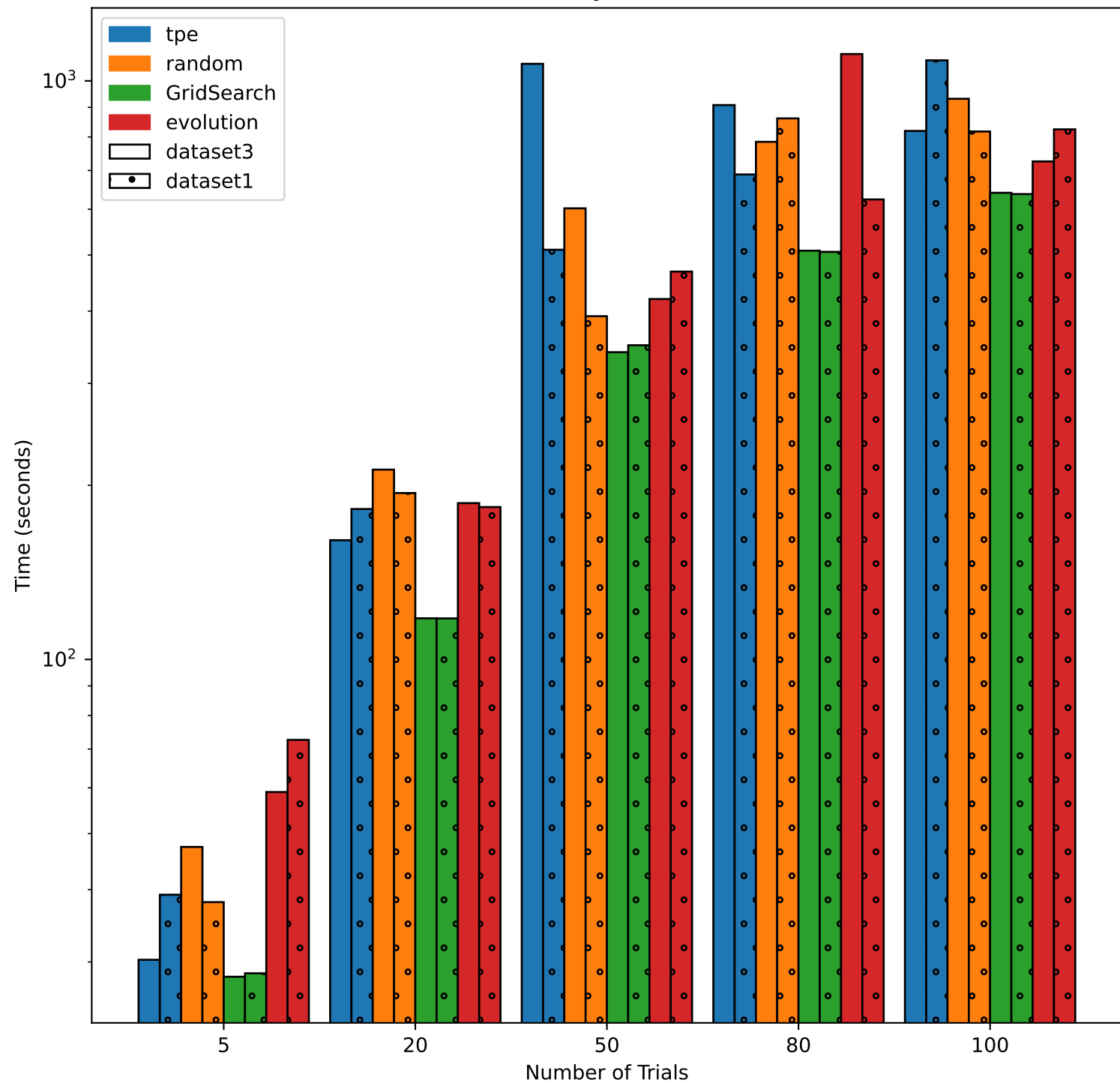
Time vs. Number of Trials by Search Method and Dataset
