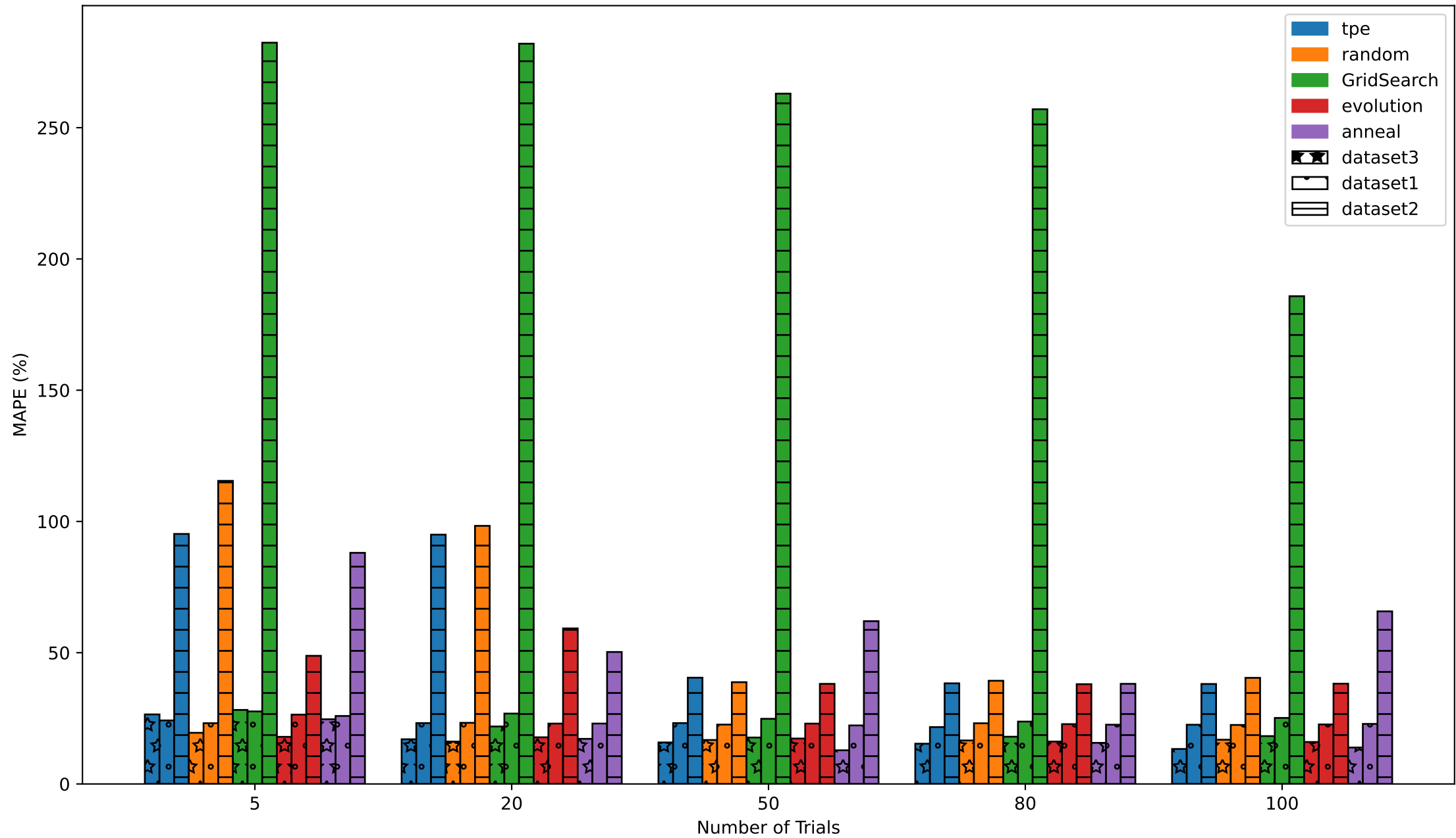
Minimum MAPE vs. Number of Trials by Search Method and Dataset
