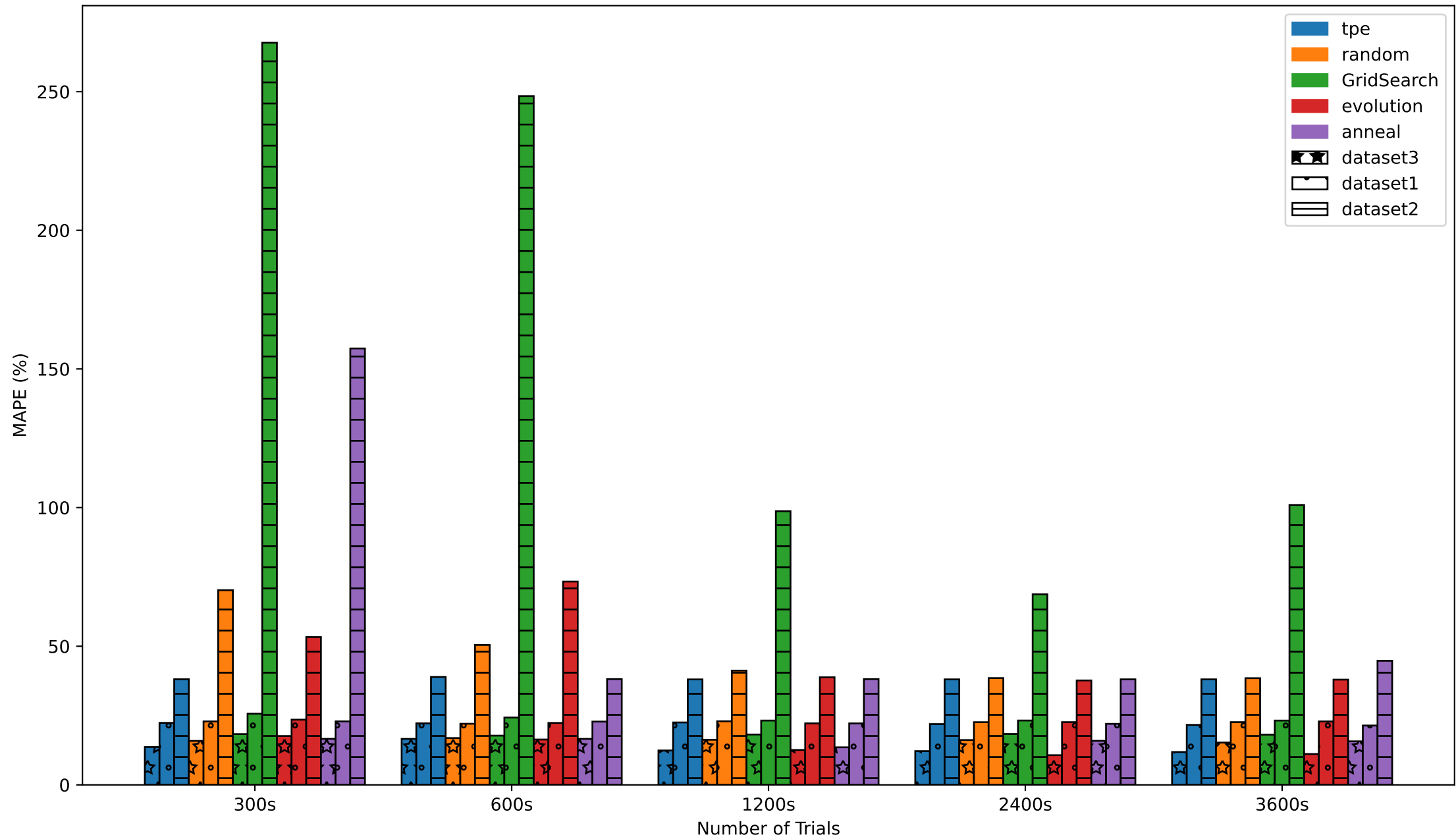
Minimum MAPE vs. exp duration by Search Method and Dataset
