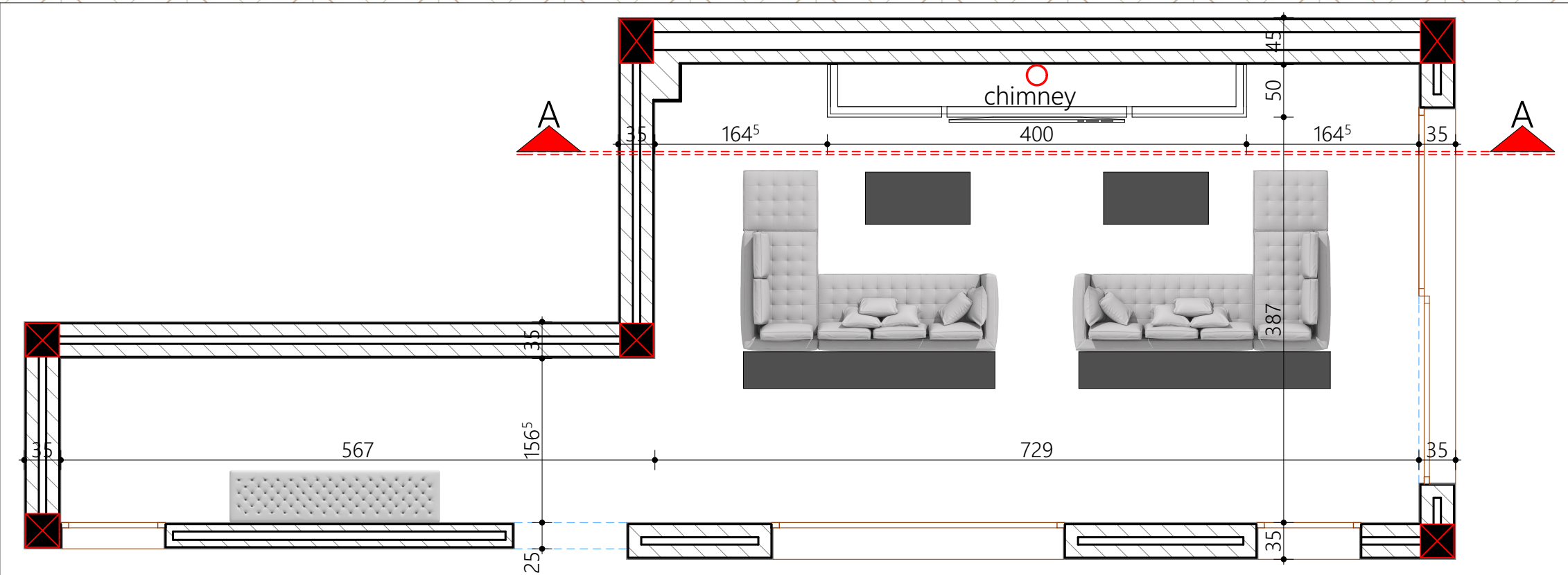
PLAN VIEW
