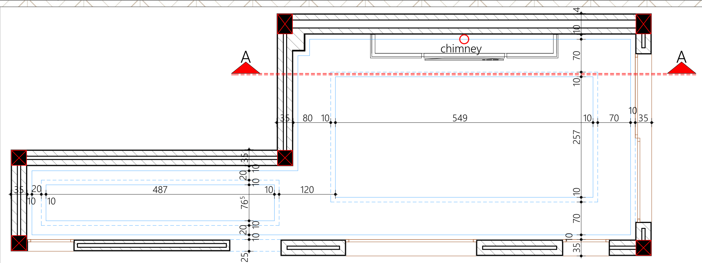
CEILING PLAN
