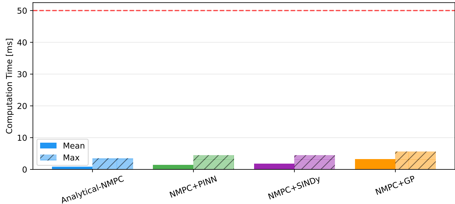
NMPC Solve Time per Step
