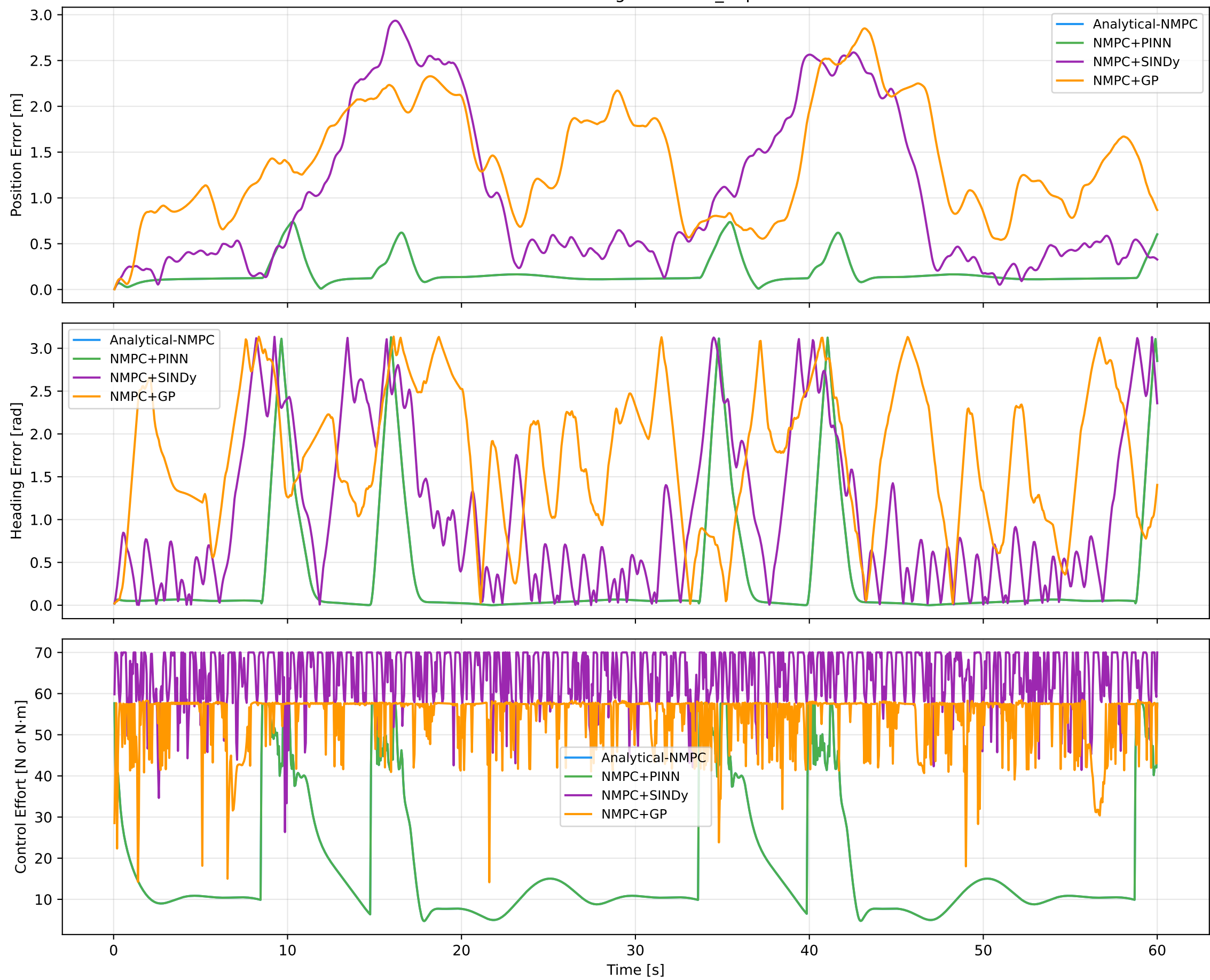
NMPC Tracking — current_25pct
