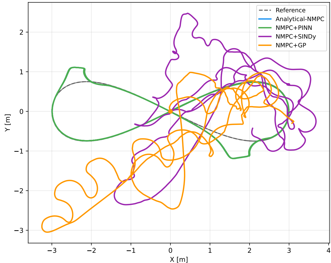
XY Trajectory — nominal
