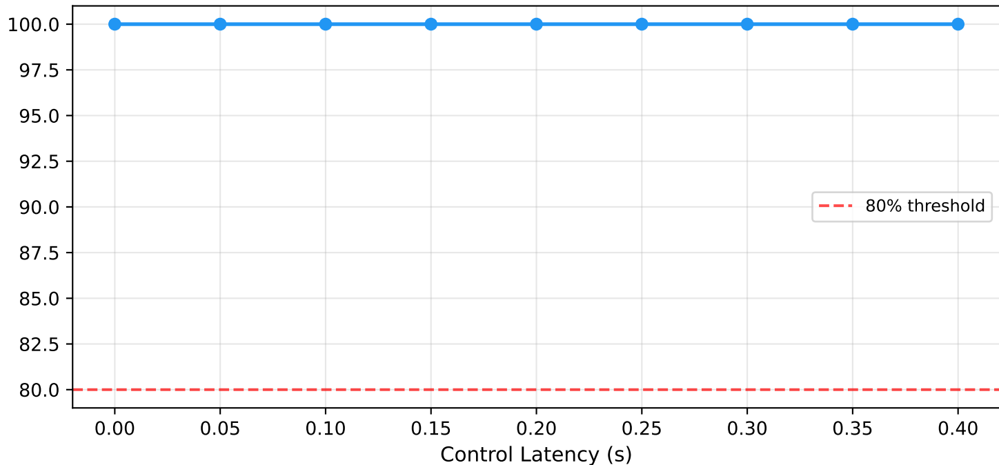
Delay Margin Analysis (Inverse Controller on BlueROV2)
