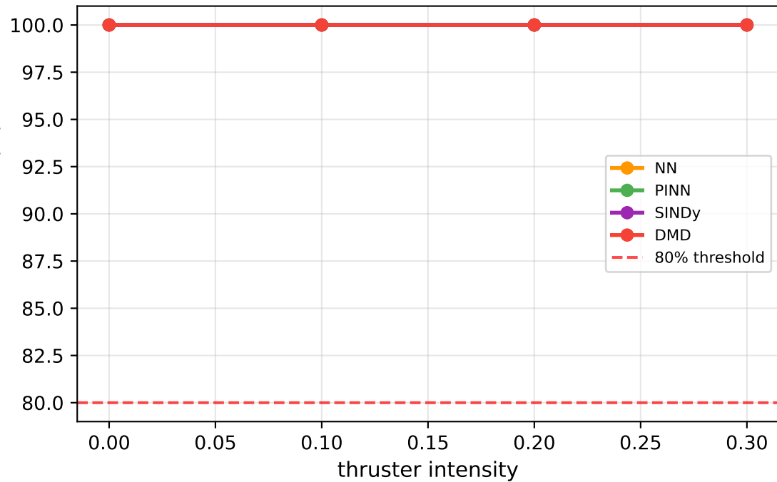
Stress Test — thruster (success rate)
