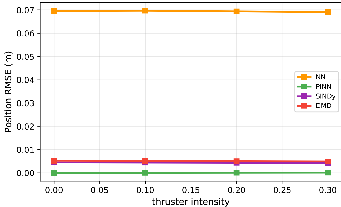
Stress Test — thruster (prediction RMSE)
