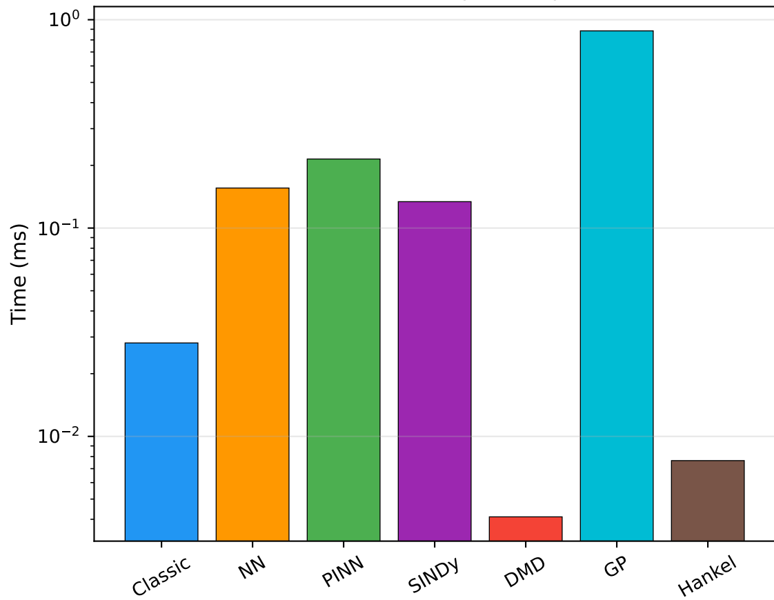
Prediction Time (per sample)
