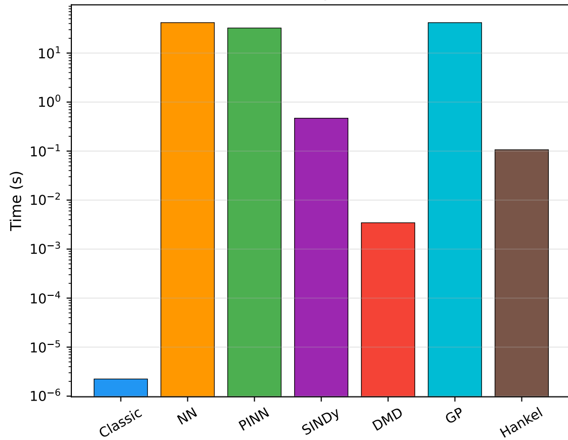
Training Time
