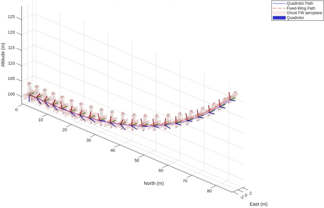
Quadrotor Tracking Fixed-Wing Trajectory (straight)
