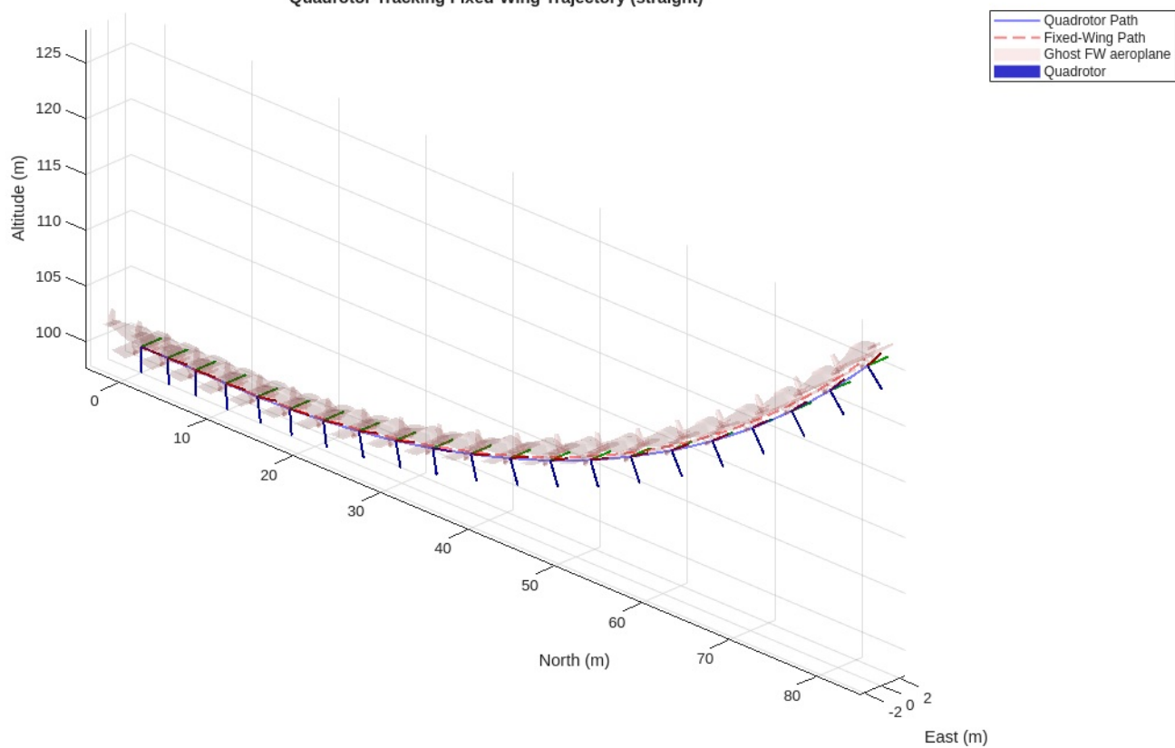
Quadrotor Tracking Fixed-Wing Trajectory (straight)
