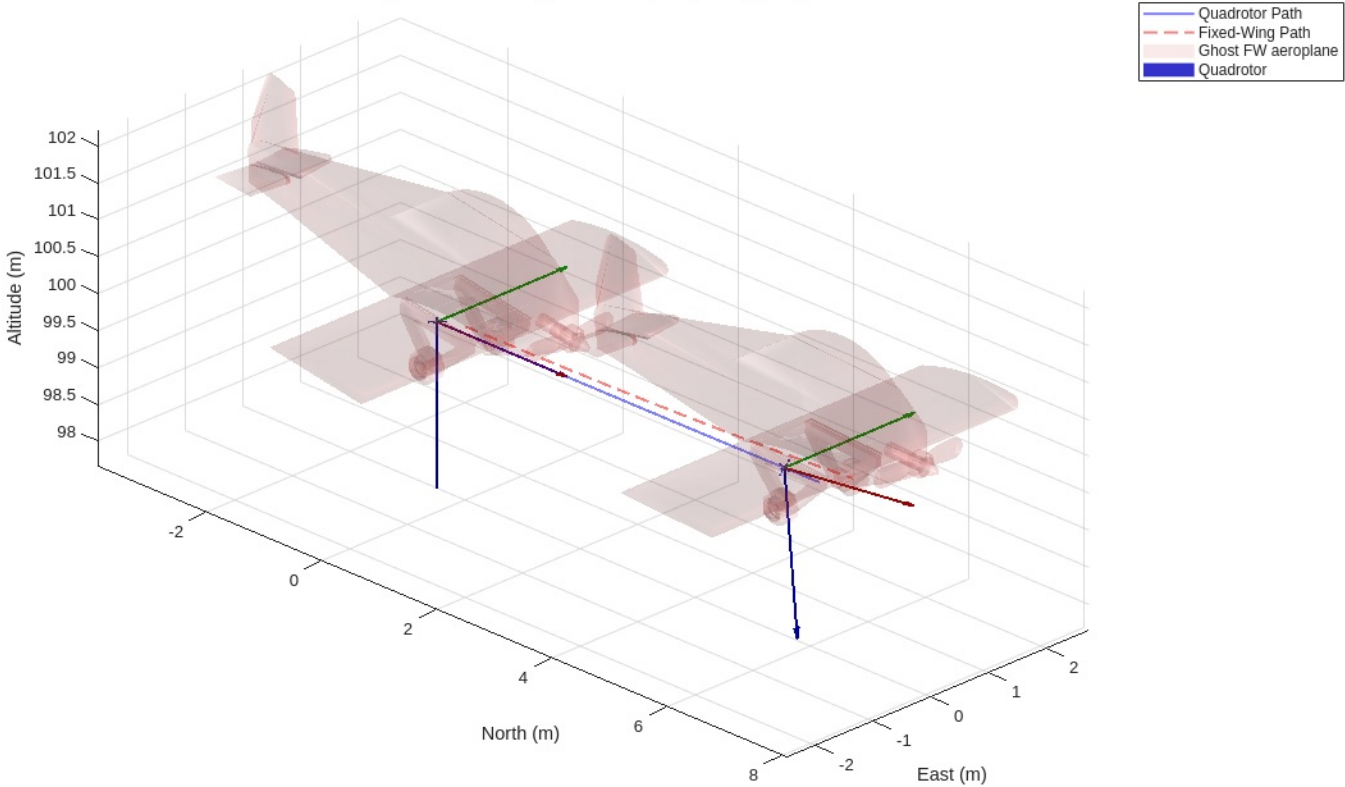
Quadrotor Tracking Fixed-Wing Trajectory (loop)
