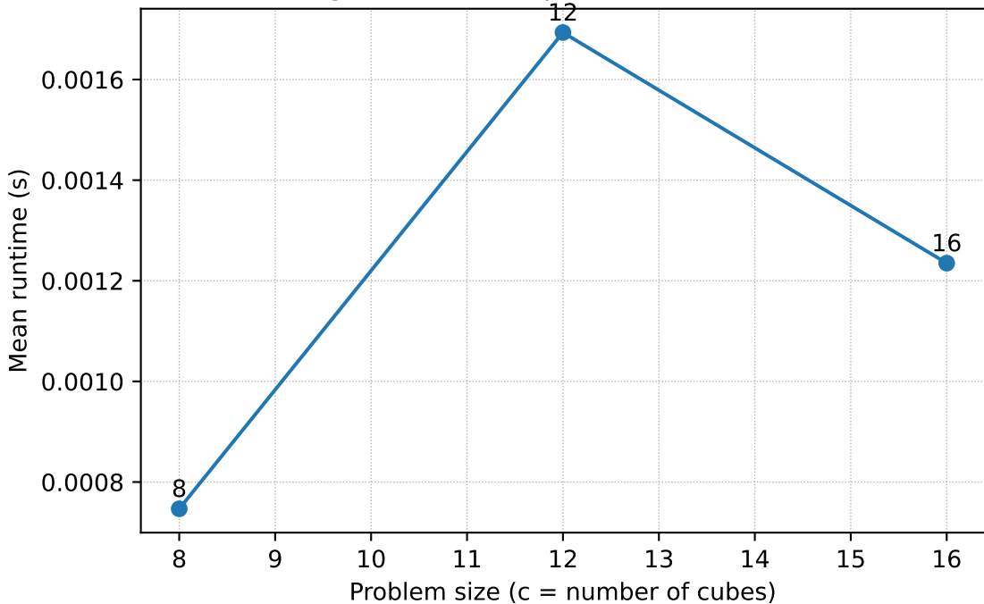
Clingo runtime vs. problem size (3DSRP)
