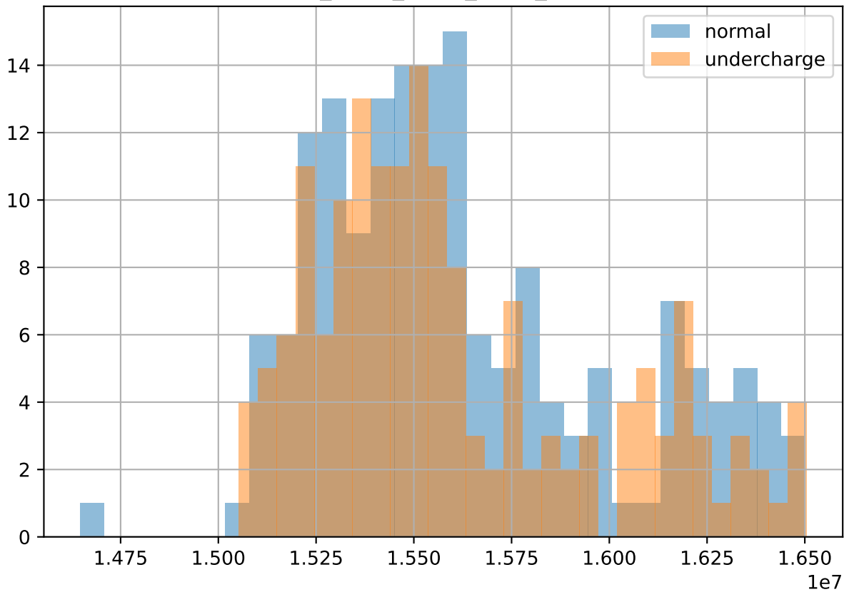
RTU_REFG_SUCTION_PRES_mean
