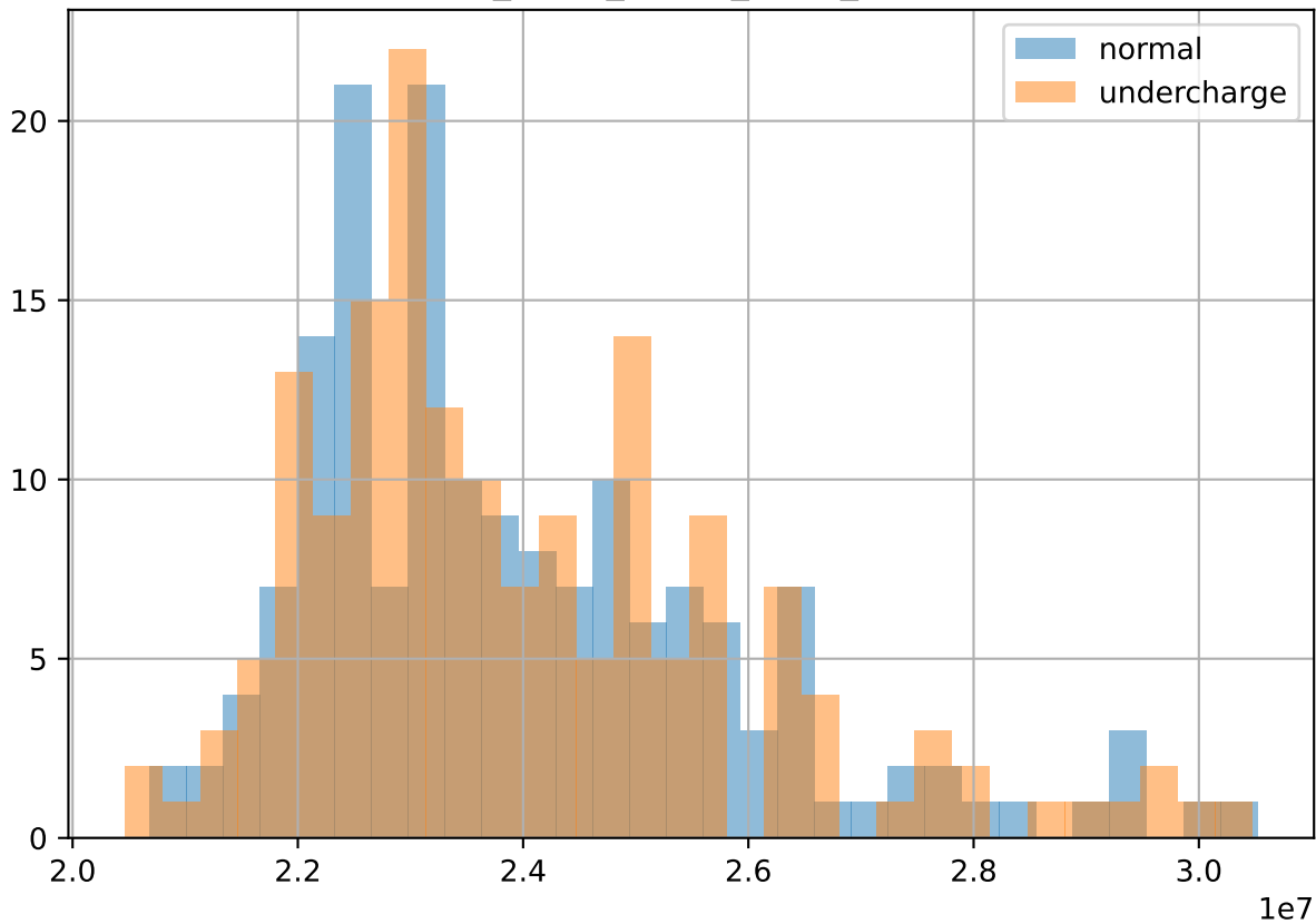
RTU_REFG_COND_PRES_mean
