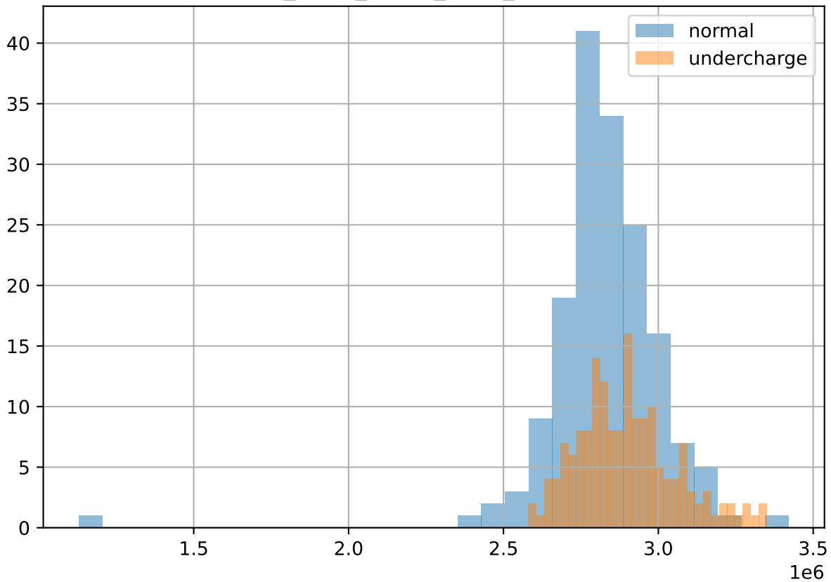
RTU_REFG_COND_PRES_oscillation
