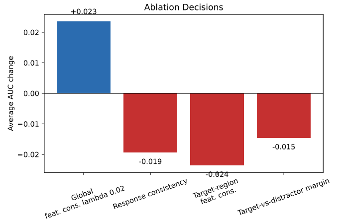
Fig. 3. Ablation decision summary. TDM is reported only as rejected negative evidence and is not part of Paper Freeze V1.
