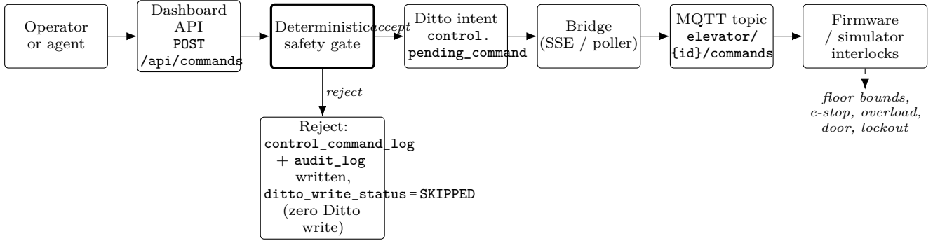
Fig. 1. Safety-gated command path. The browser, workflows, and optional LLM never publish device commands directly. Accepted intent is persisted as Ditto command intent and forwarded by the bridge; rejected commands are logged for audit but produce zero Ditto writes ( ditto_write_status = SKIPPED ). The firmware or simulator applies local interlocks before actuation.
