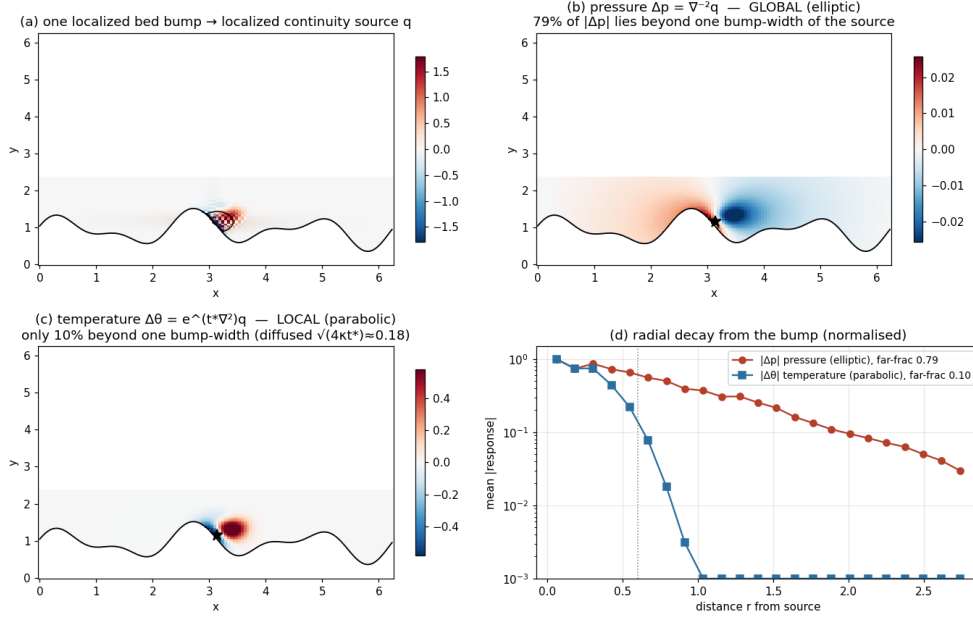
Part 9 — geometry shapes the GLOBAL pressure, only the LOCAL temperature (same localized bed bump; elliptic vs parabolic response)
