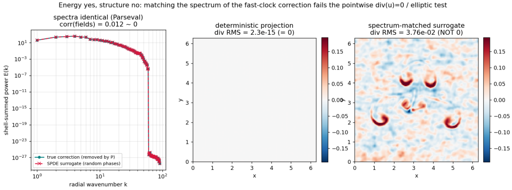
FIG. 11. Spectrum-matched surrogate test. A phase-randomized field with the identical power spectrum as the true projection correction (Parseval-exact) fails to reproduce the correction pointwise: ensemble-median correlation |r| = 0.07 ( n = 100 ), and the divergence constraint is left unrepaired (RMS \nabla \cdot \mathbf{u} = 3.7 \times 10^{-2} , compared to 2 \times 10^{-15} for the true projection).
