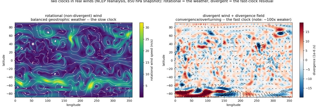
FIG. 12. NCEP/NCAR winds, one analysis day. Left: rotational wind (synoptic highs, lows, and jets). Right: divergent wind (weak, confined to convergence and overturning zones).
