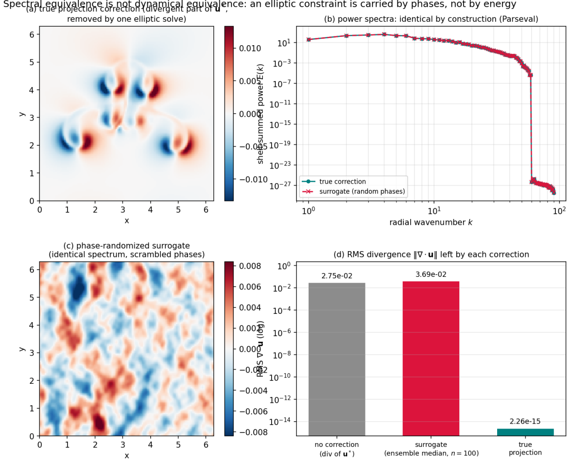
FIG. 1. The surrogate test in one figure. (a) The true projection correction: the divergent part of the intermediate velocity \mathbf{u}^* that a single elliptic solve removes. (b) Power spectra of the true correction and of a phase-randomized surrogate—identical by construction (Parseval-exact). (c) The surrogate correction field: the same spectrum, scrambled phases. (d) RMS divergence left by no correction ( 2.7 \times 10^{-2} ), by the surrogate (ensemble median 3.7 \times 10^{-2} , n = 100 ), and by the true projection ( 2 \times 10^{-15} ). Spectral equivalence is not dynamical equivalence: a field that matches the correction’s power spectrum does not reproduce its action as a constraint.
