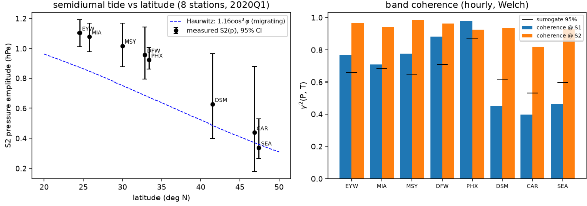
FIG. 3. Left: semidiurnal pressure-tide amplitude versus latitude at eight ASOS stations with bootstrap 95% confidence intervals, compared to the Haurwitz migrating-tide climatology (dashed curve). The monotonic equator-to-pole decay is the signature of a global resonance. Right: band-resolved coherence between hourly pressure and temperature—high at the shared solar lines, at the surrogate noise floor off-line.
