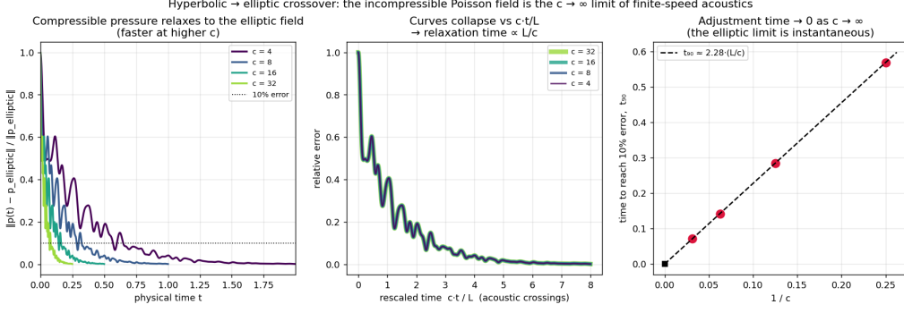
FIG. 7. Relaxation of the compressible pressure field to the elliptic (Poisson) solution for several sound speeds. All curves collapse in the rescaled time ct/L , with t_{90} \approx 2.3 L/c .
